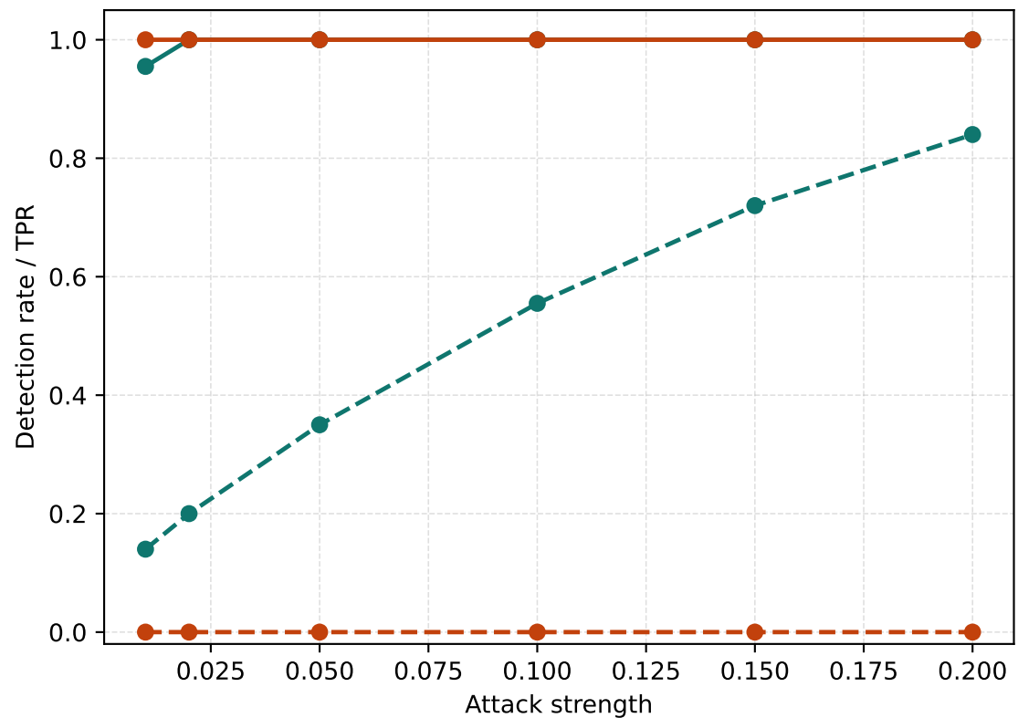
Experiment C strength sweep: color encodes verifier; line style encodes attack
