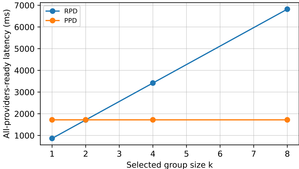
Selective delivery latency (LAN, 100MB)
