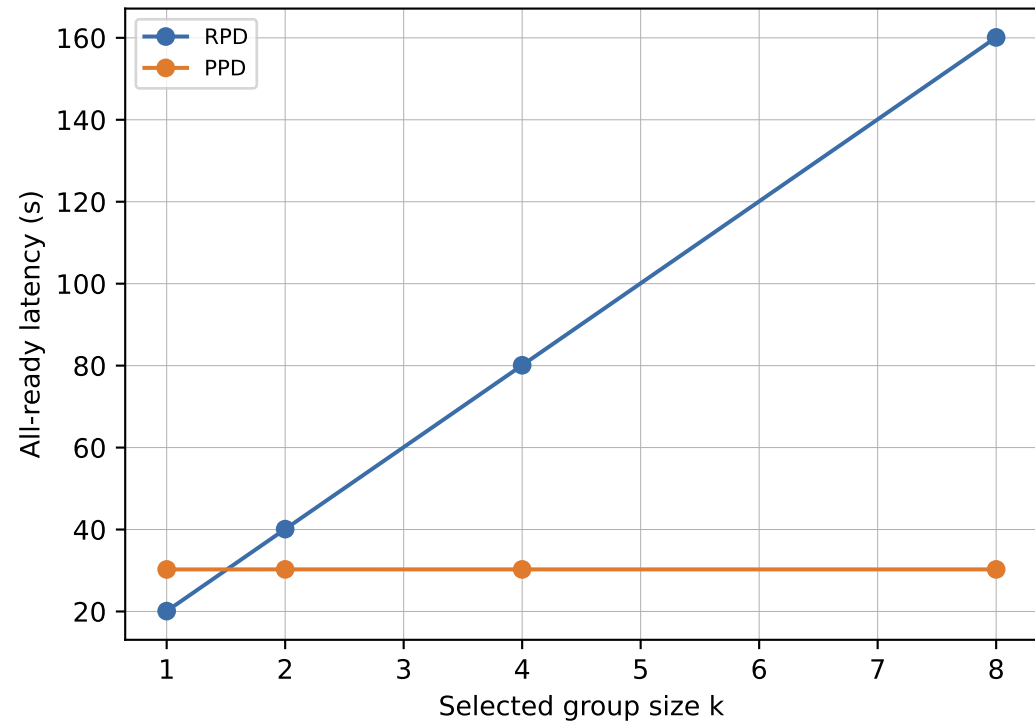
WAN delivery latency
