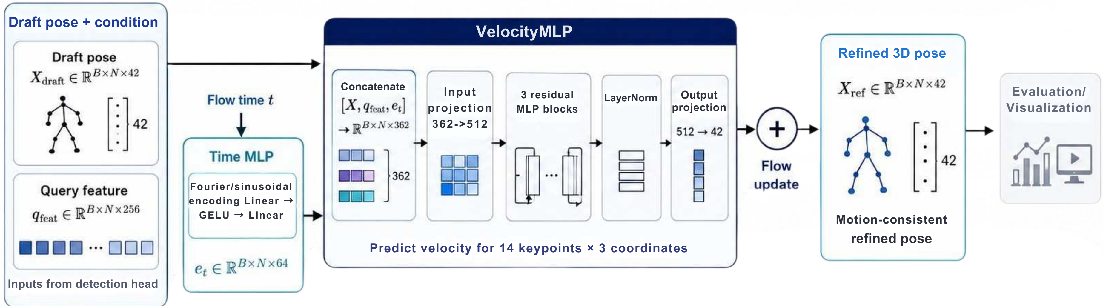
Residual pose refinement with Rectified Flow
