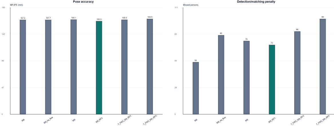
Fig. 6. Flow solver analysis showing MPJPE and unmatched-person count.
