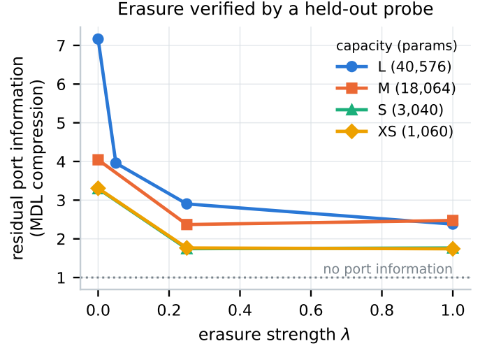
Figure 3: Residual destination-port information in the latent, measured by a probe fitted after training on frozen representations. 1.0 denotes no recoverable information.
