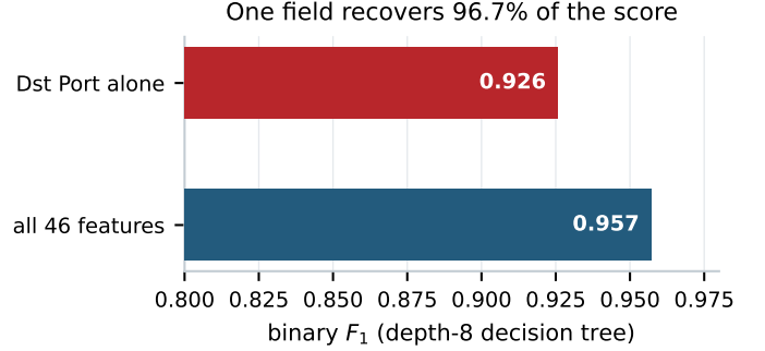
Figure 1: The destination port alone recovers almost the entire detection score available from all 46 features.
