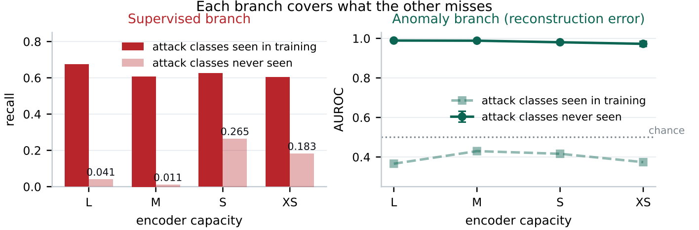
Figure 2: The two branches are complementary. The supervised head detects attack classes seen in training but is near-blind to novel ones; the reconstruction-error branch is close to perfect on novel classes and below chance on seen ones, because seen attacks lie inside the distribution it was fitted to. Error bars are one standard deviation over seeds.
