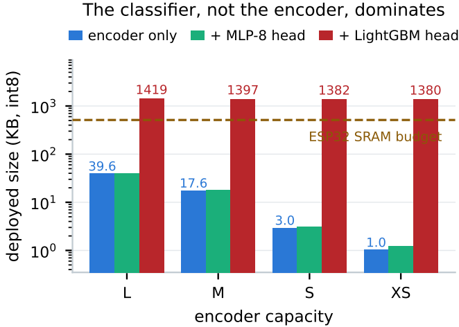
Figure 4: Where the bytes go. The encoder is small at every capacity; the classifier that must ship with it is not. Only the MLP-8 configuration fits an ESP32-class budget.
