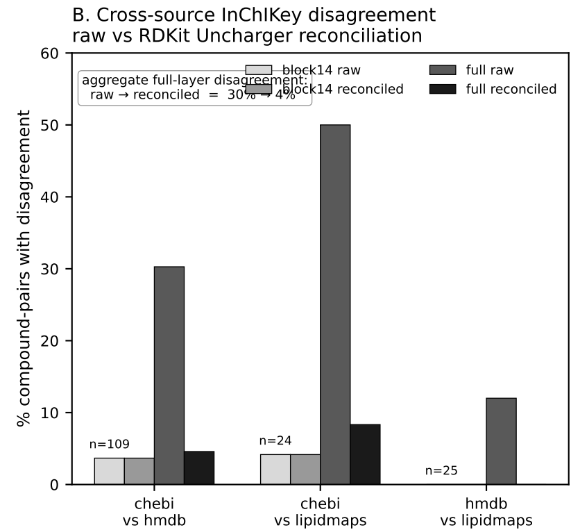
Fig. 3 (v2, refined). PA-method disagreement (Panel A) motivates ConcordMet reconciliation; cross-source InChIKey disagreement (Panel B) is reduced 30% → 4% (full-layer aggregate) by RDKit Uncharger + tautomer canonicalization.
