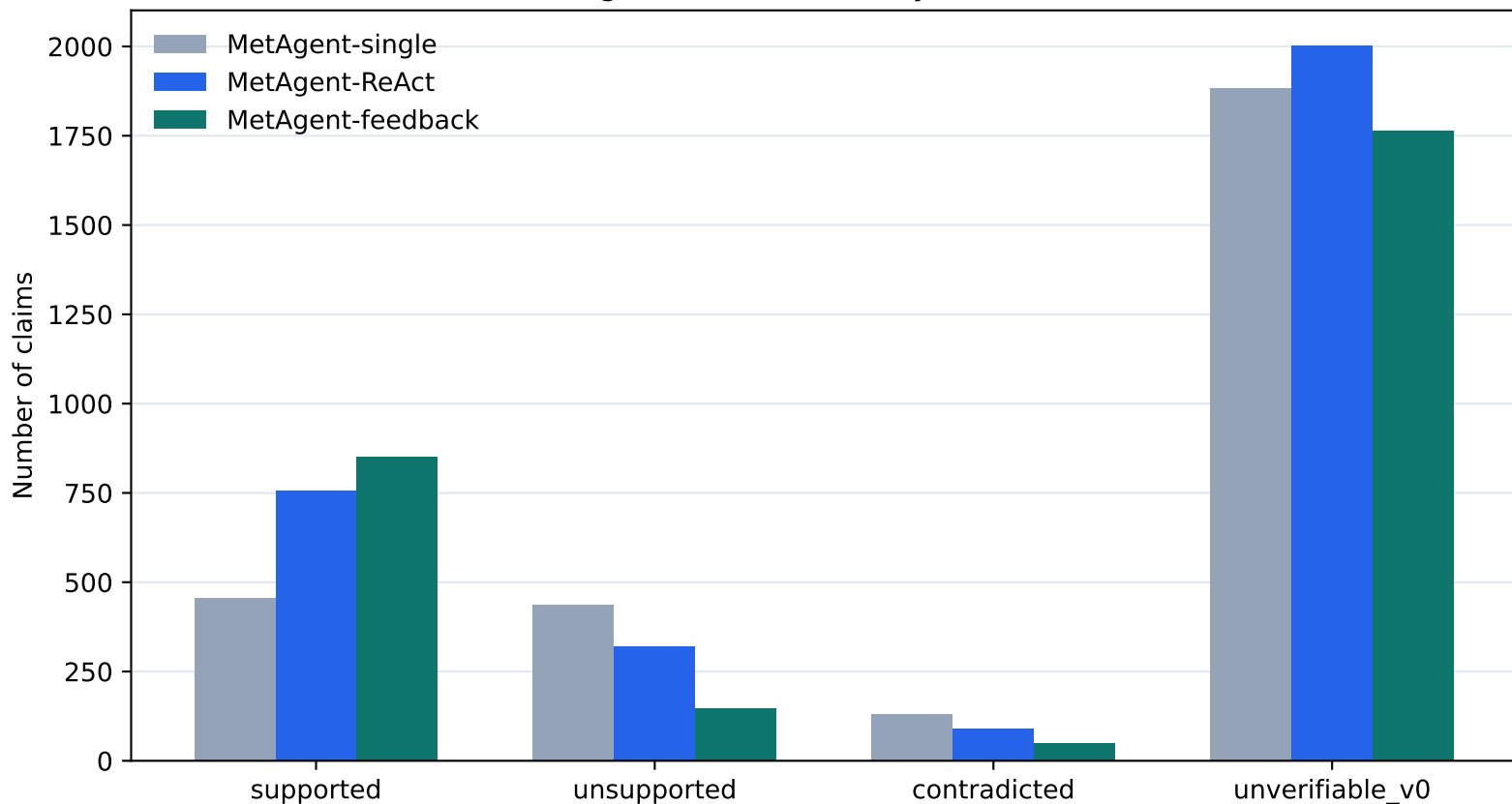
MetAgent verdict totals by architecture
