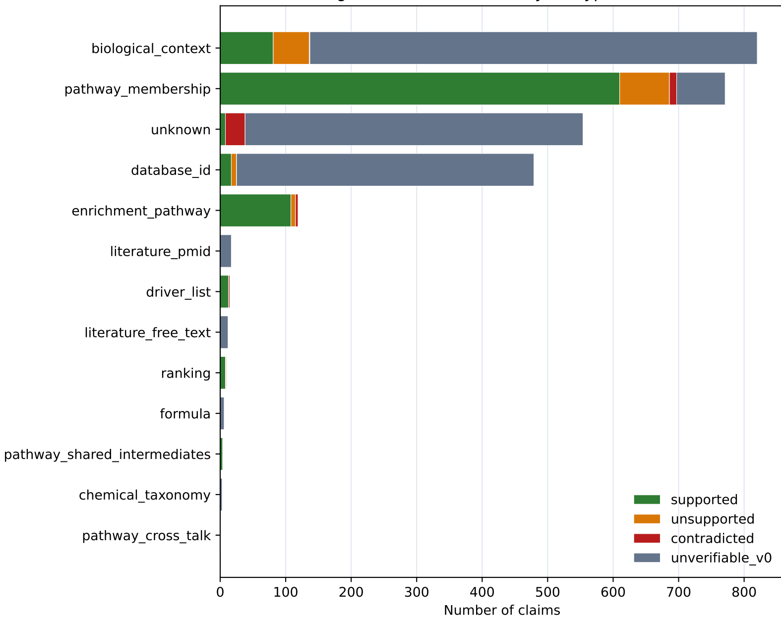
MetAgent D3 v4 final claims by subtype and verdict
