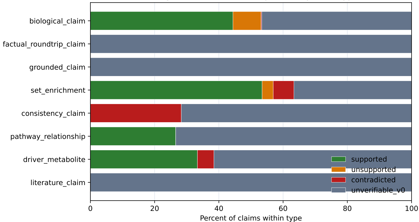
MetAgent D3 v4 verdict composition by claim type
