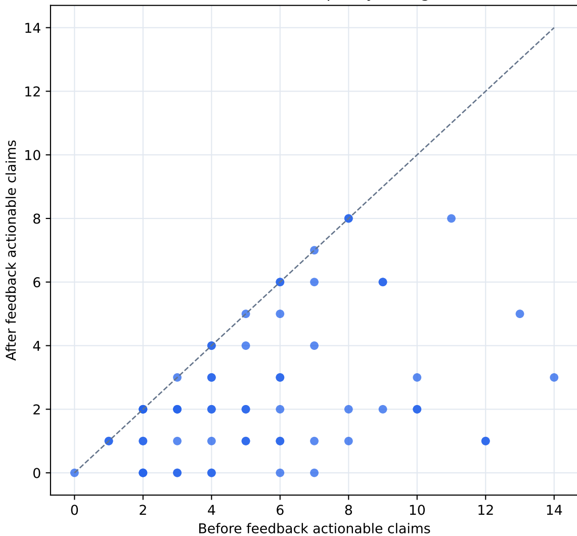
Per-task verifier quality change
