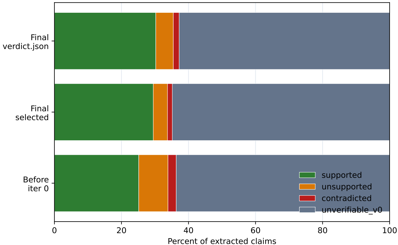
Verifier verdict composition within feedback run
