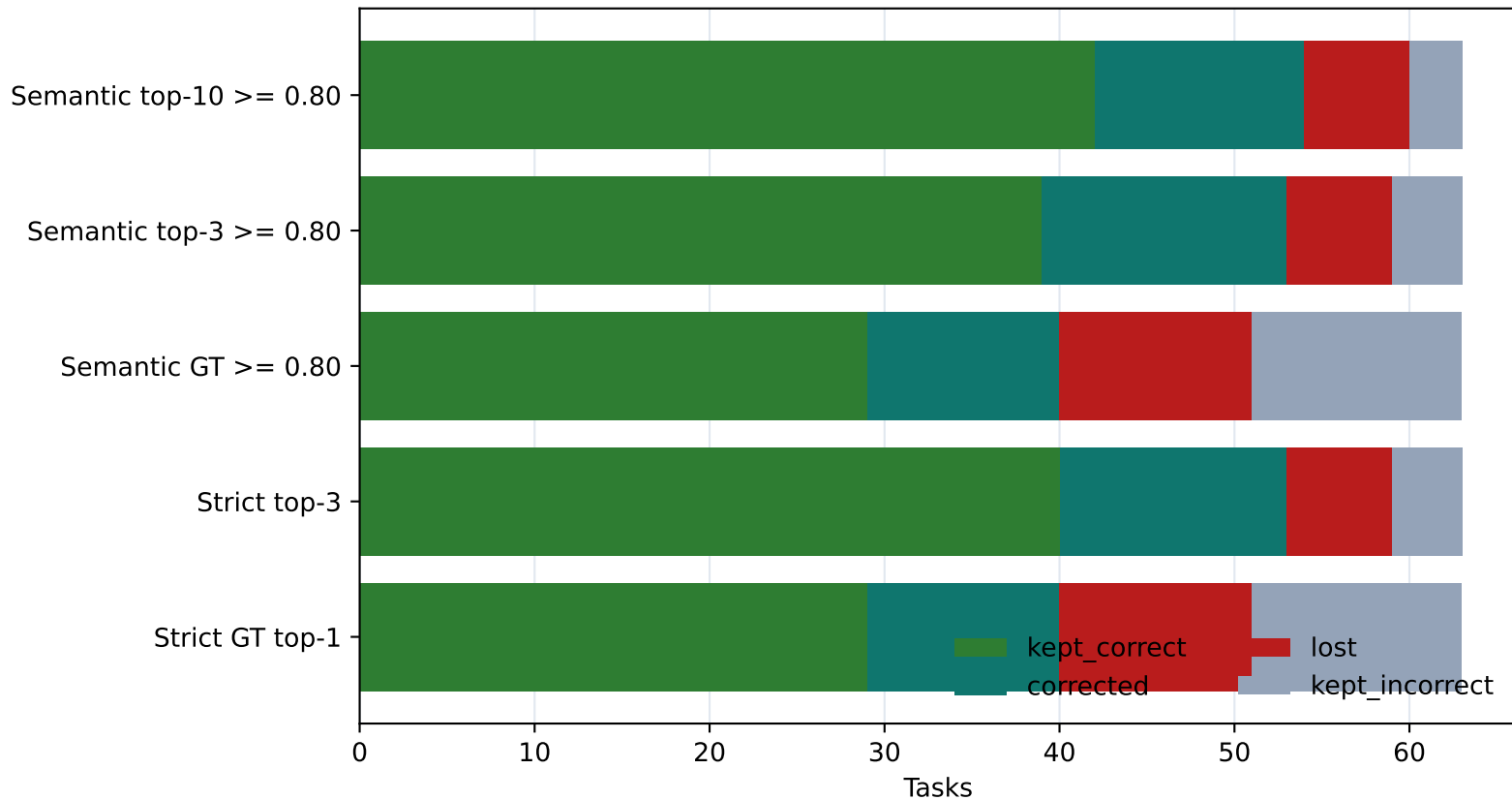
Task-level transitions after feedback
