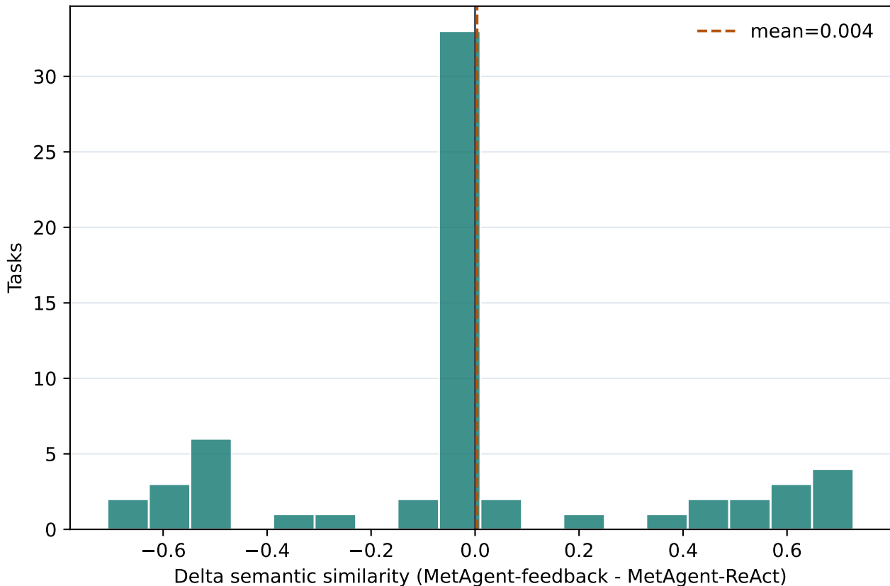
Semantic pathway-similarity change after feedback
