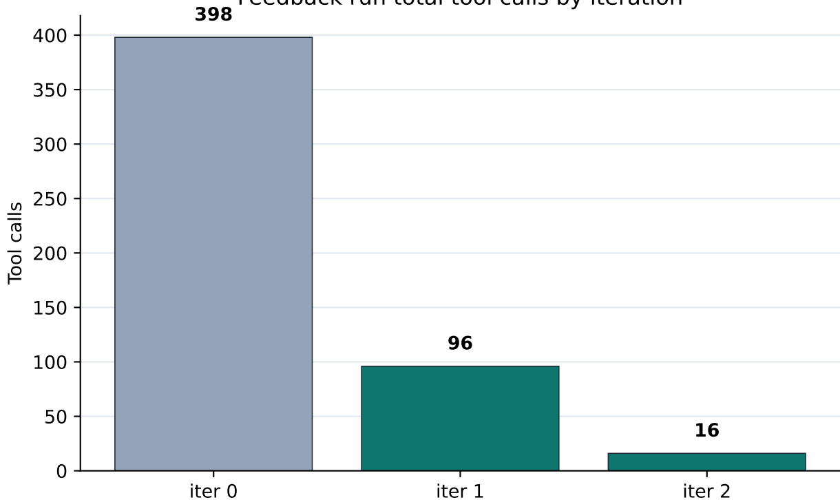
Feedback run total tool calls by iteration
