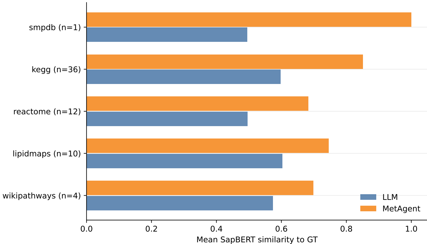
Performance by ground-truth pathway source
