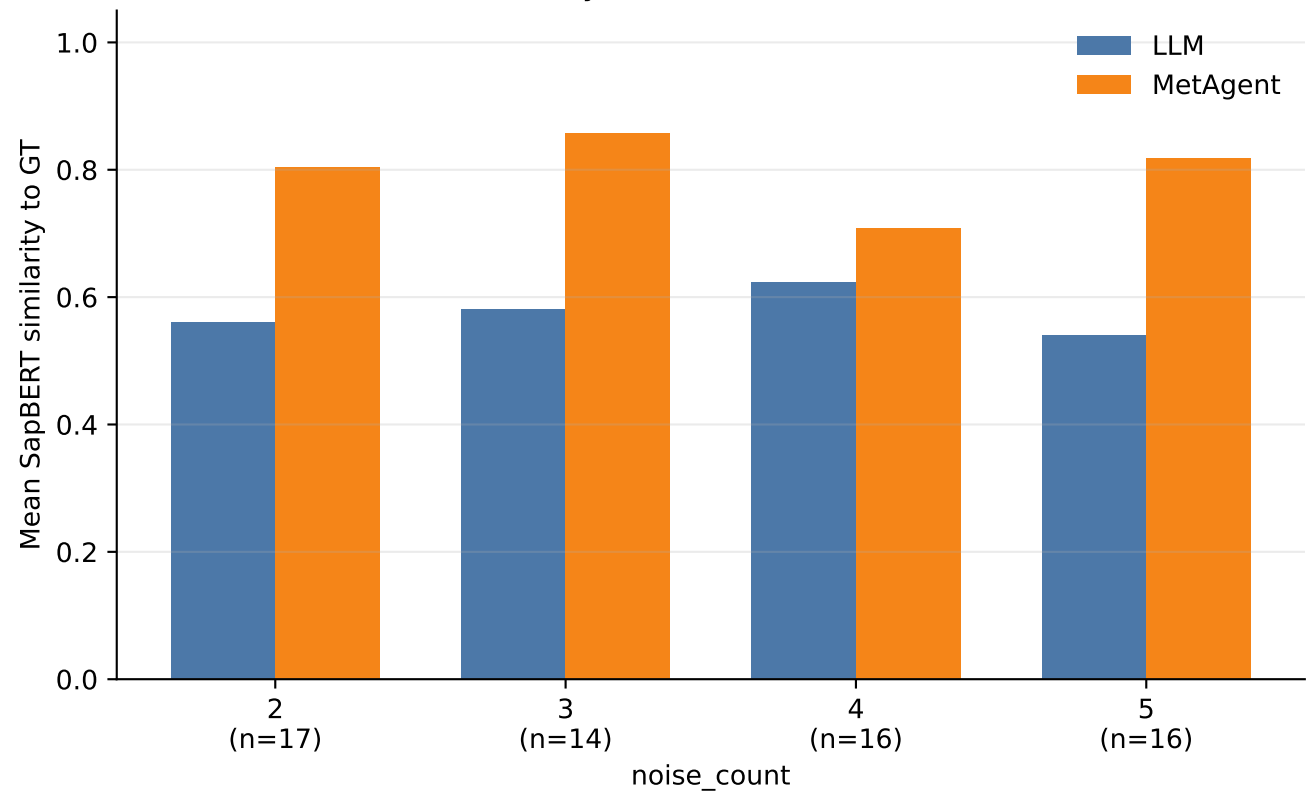
Performance by number of noise metabolites
