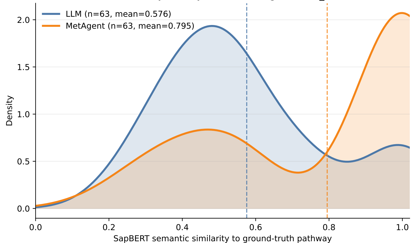
Semantic similarity density: LLM vs MetAgent (with_lit, D3 full)
