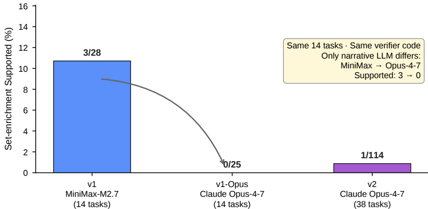
c LLM-style sensitivity: same verifier, swap narrative LLM
