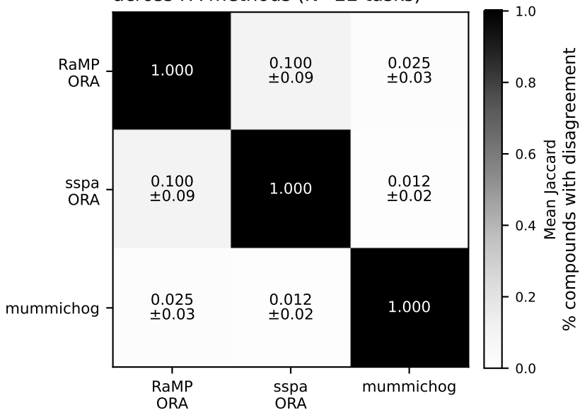
A. Top-10 pathway Jaccard across PA methods (N=22 tasks)
