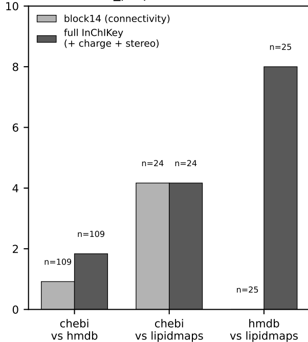
Fig. 3 (preliminary). PA-method disagreement and cross-source ID disagreement motivate ConcordMet reconciliation. Refined Fig. 3 v2 with full RDKit Uncharger normalization in W4. B. Cross-source InChIKey disagreement (RaMP chem_props, 3 sources)
