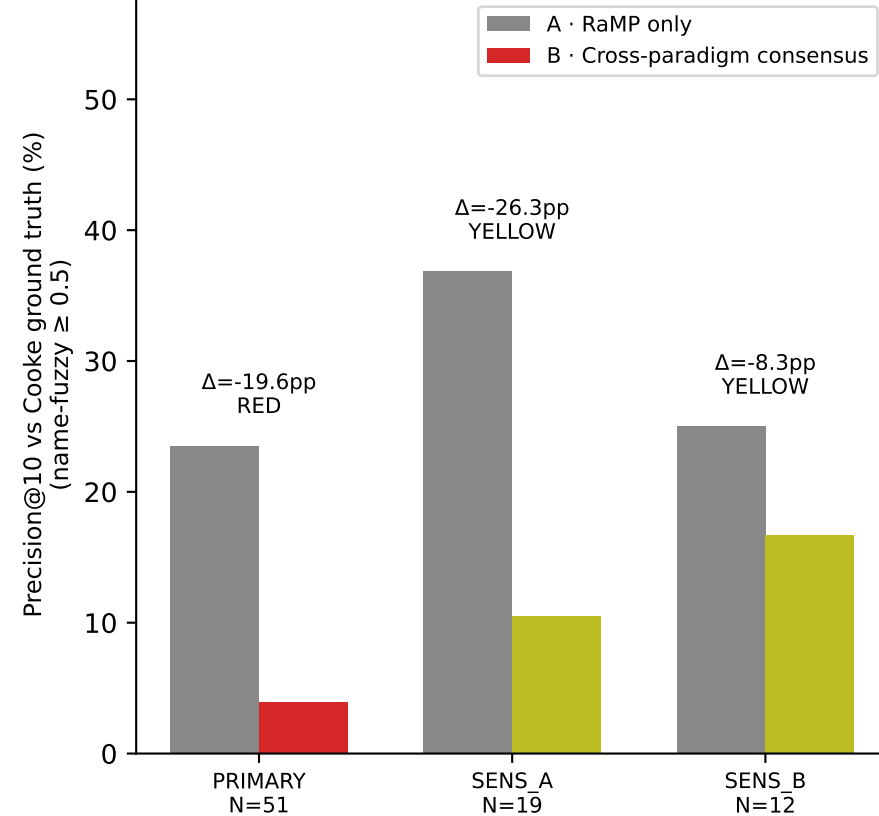
C · Gate-2 precision lift (A=baseline · B=consensus)
