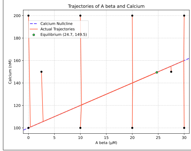
Figure 4: Phase portrait
