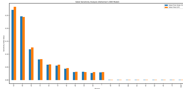
Figure 1: First and Total order indices at N = 2^{10}
