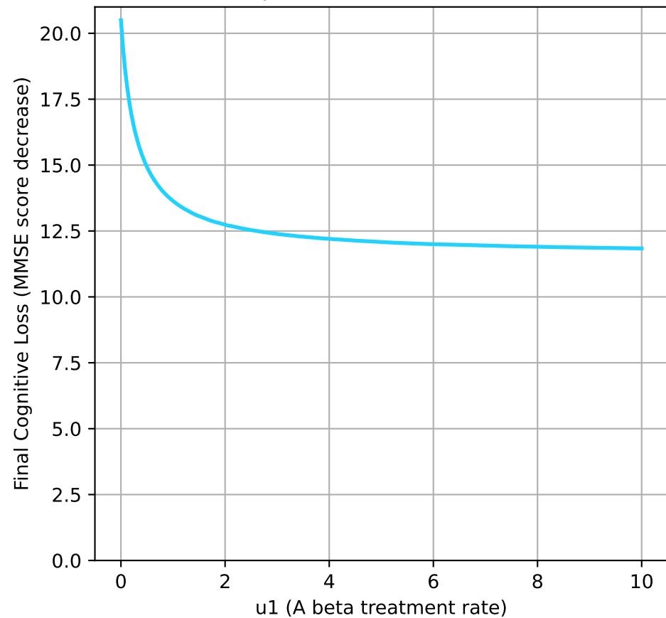
Impact of u_1 on C at t=50
