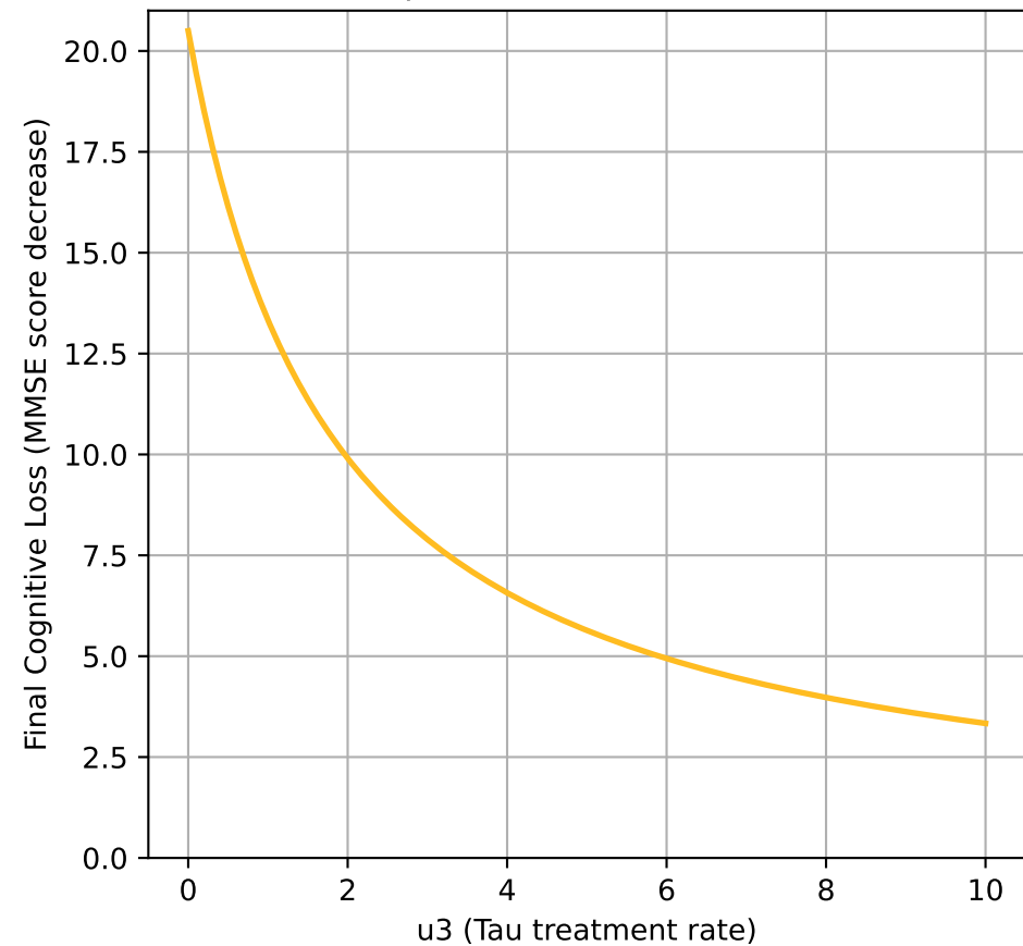
Impact of u_3 on C at t=50
