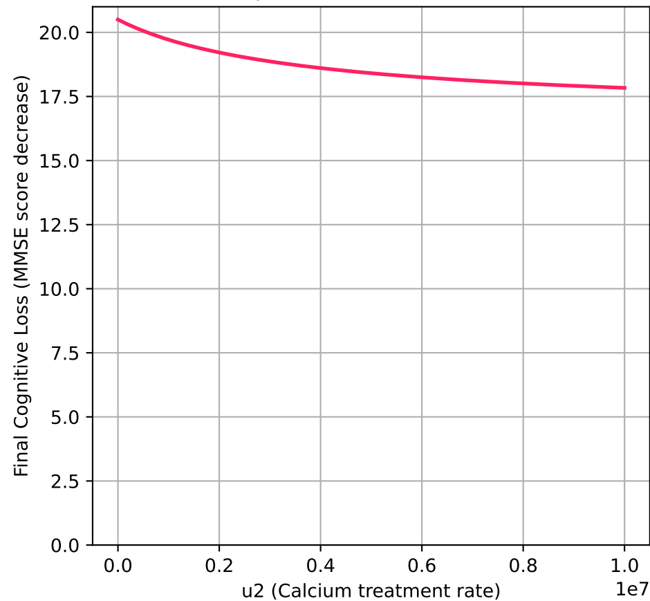
Impact of u_2 on C at t=50
