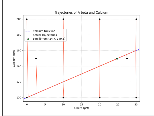
Figure 2: Phase portrait
