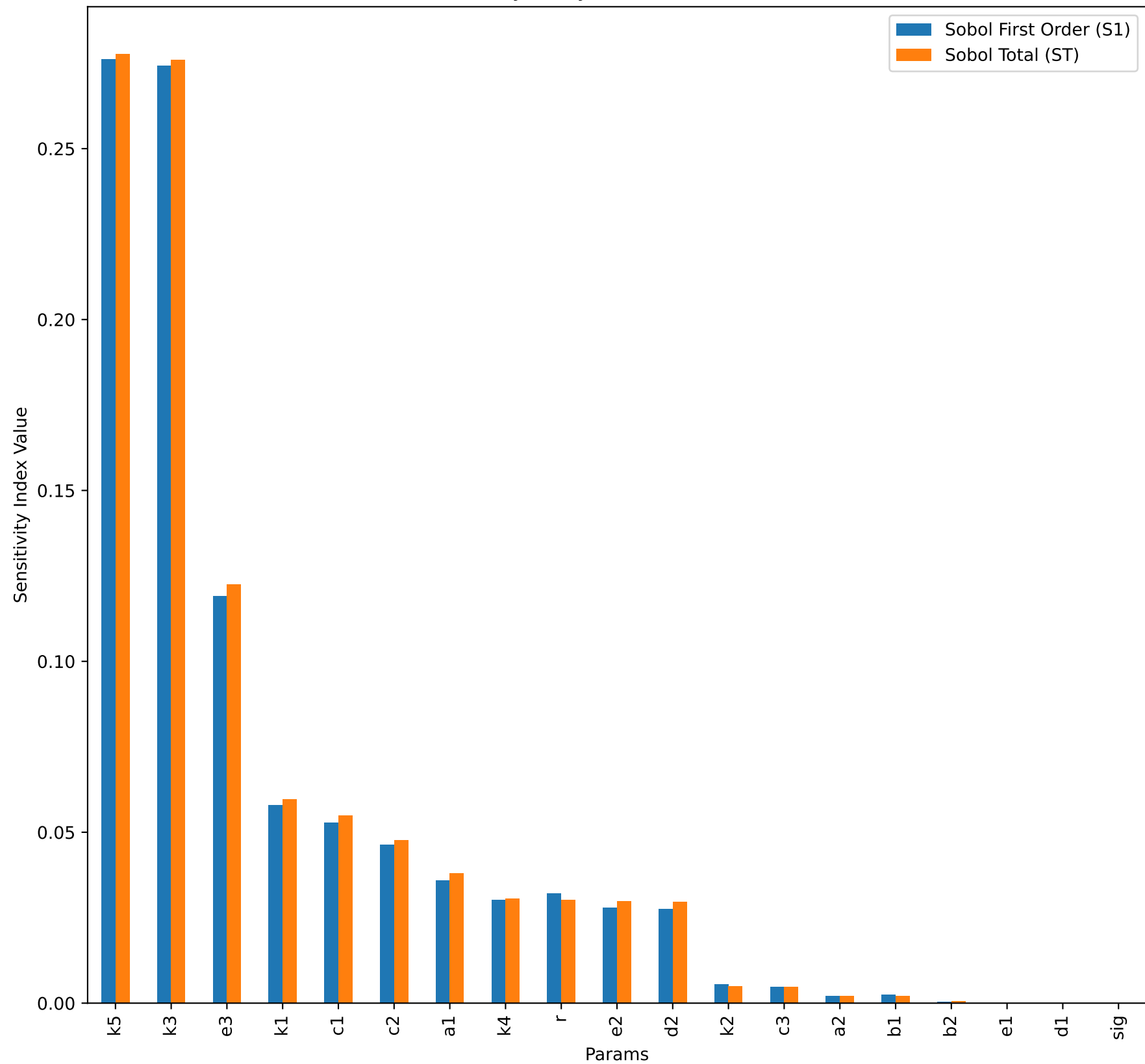
Sobol Sensitivity Analysis (Alzheimer's ODE Model)
