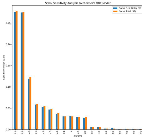
Figure: Visualization of Sobol Orders
