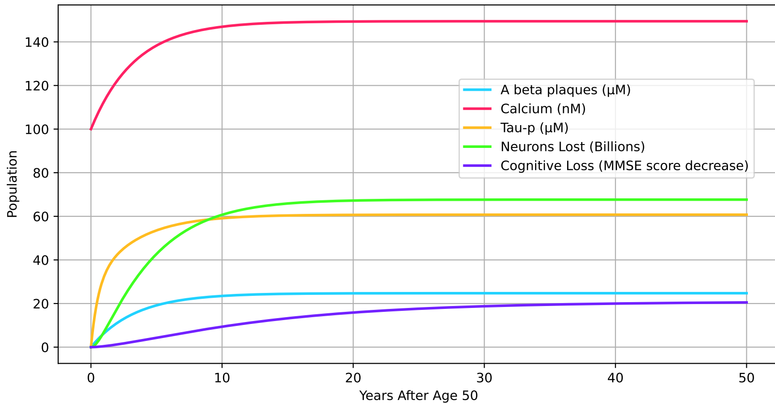
Alzheimer's ODE Simulation
