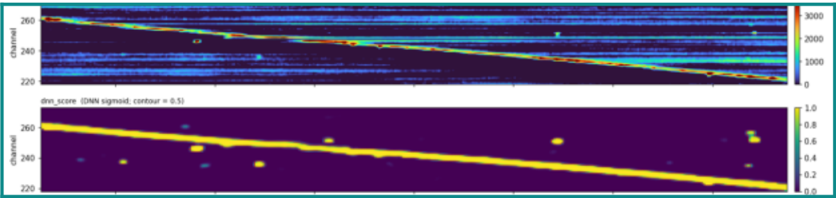
DNN-ROI: charge → CNN score
