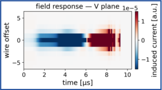
field-response kernel (V)
