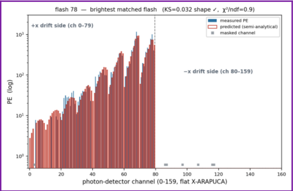
Q/L light pattern — flash 78 (measured vs semi-analytical prediction)
