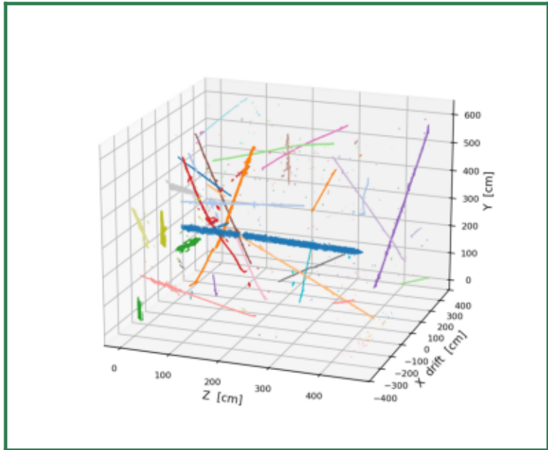
clustering result — clusters coloured (evt 983)
