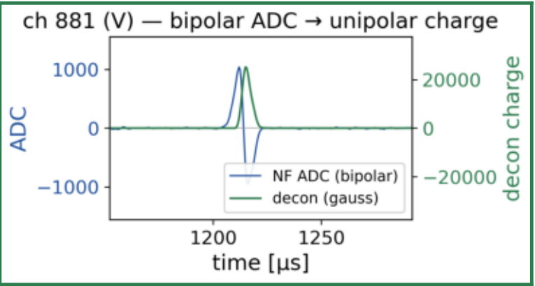
NF ADC → deconvolved charge
