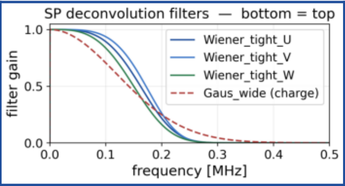
SP deconvolution filters
