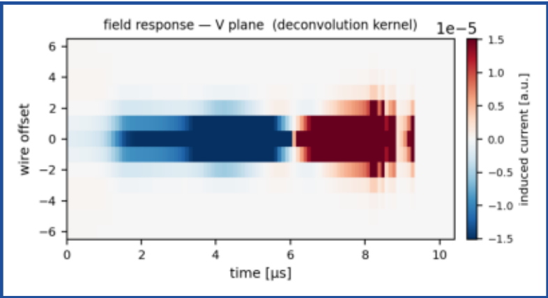
field-response kernel (V)
