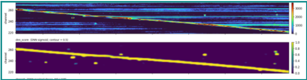
DNN-ROI: deconvolved charge → CNN score (data)
