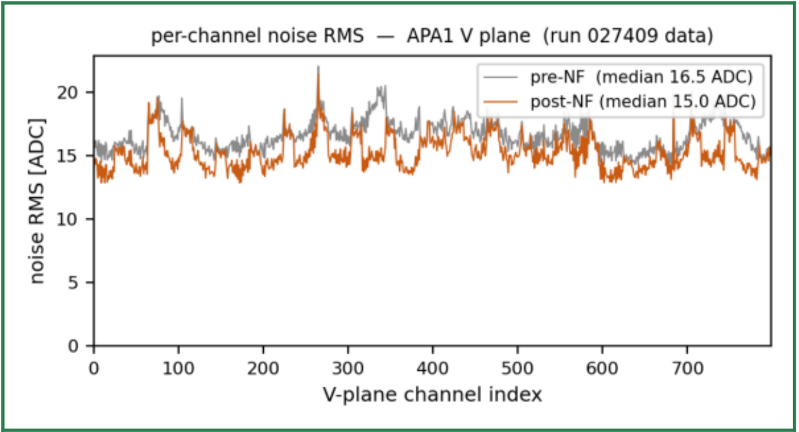
noise RMS: pre-NF → post-NF (data)
