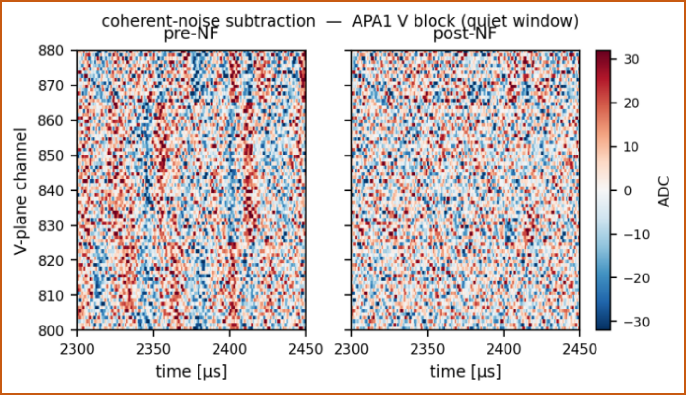
coherent-noise subtraction (data)
