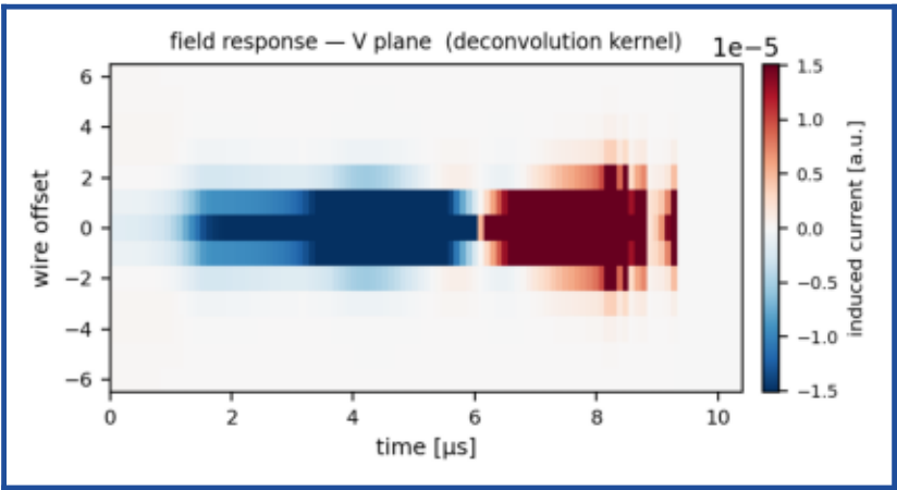
field response kernel (V)
