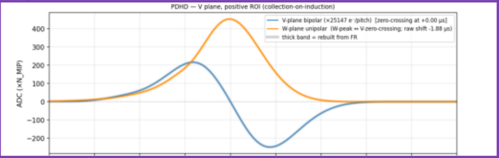
L1SP response bases (V bipolar / W unipolar)
