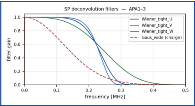
SP deconvolution filters
