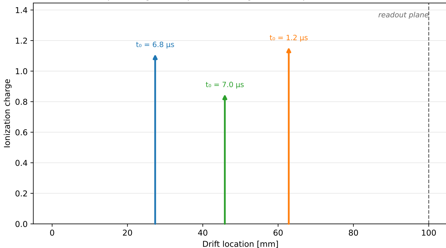
Point-like ionization depositions at their drift locations (spike height = deposited charge; label = production time)
