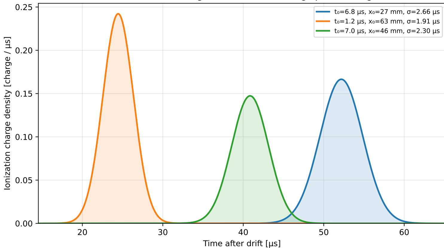
Diffused charge arriving at the readout plane ( x = 100 mm) (each Gaussian integrates to the matching spike's charge)
