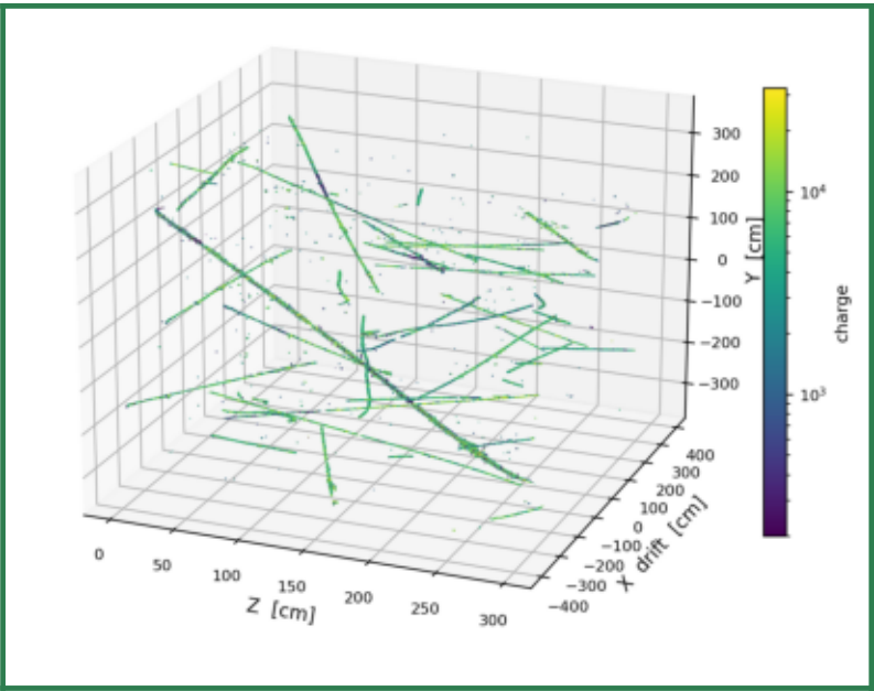
full event 3-D charge display (Bee) — deghosted result
