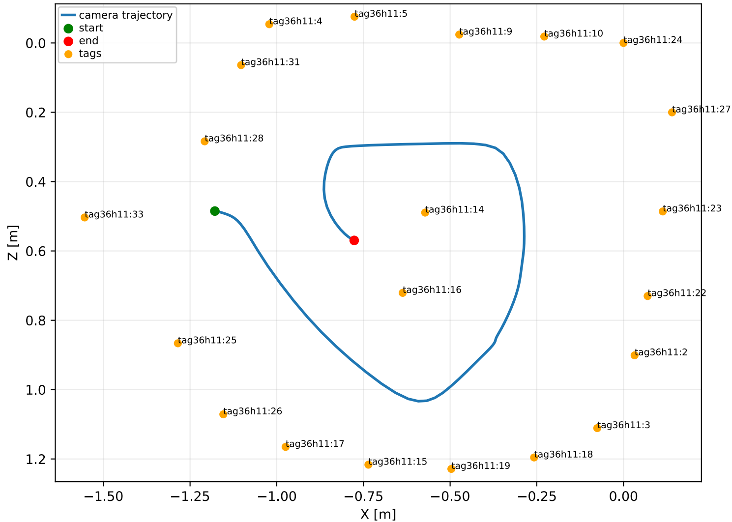
AprilTag Environment Reconstruction and Estimated Trajectory
