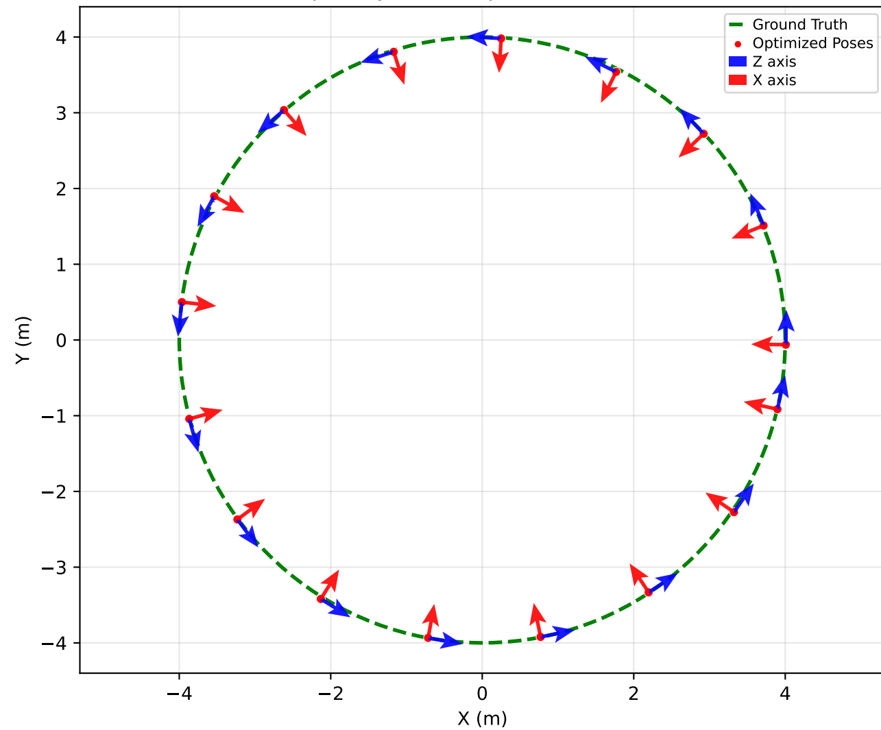
Camera Trajectory: GT vs Optimized with 10 cm noise
