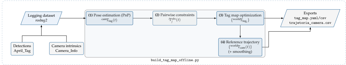
Figure 3.3. Architecture of the offline recording pipeline.
