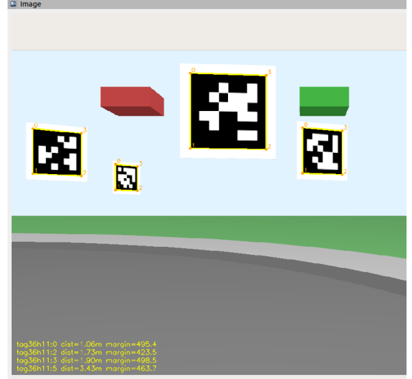
(b) AprilTag detection in the simulated environment.
