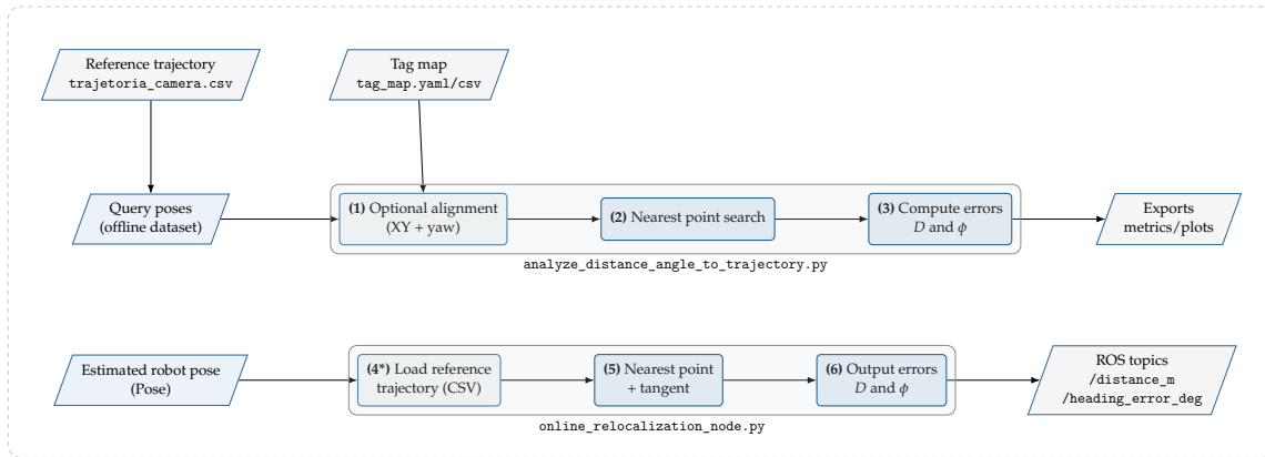
Figure 3.4. Architecture of the relocalization pipeline with separated offline analysis and online execution. Step (4*) loads the reference trajectory generated in the recording phase. Both workflows compute the distance to the reference trajectory D and the heading deviation \phi as control-oriented outputs.
