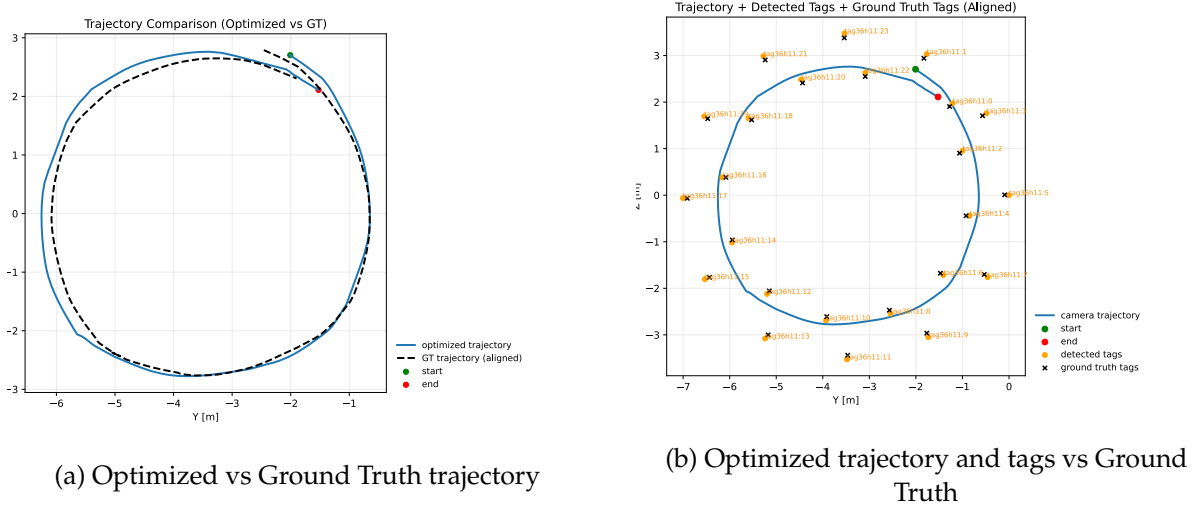
Figure 4.4. Comparison between optimized reconstruction and ground-truth configuration.
