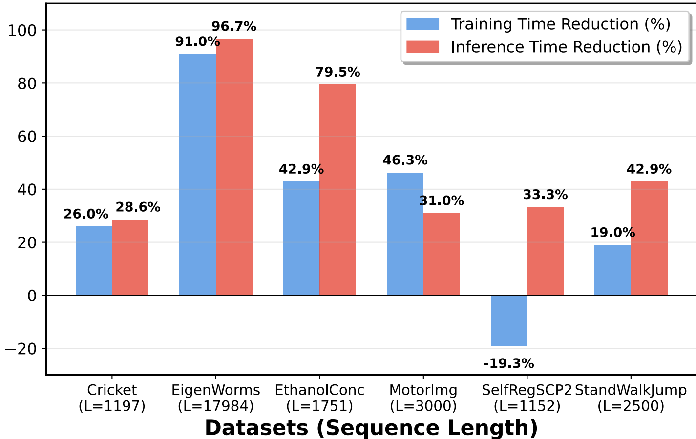
Runtime Reduction (%)
