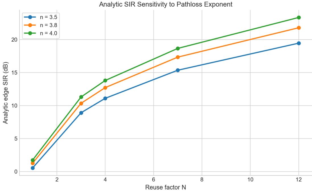
Fig. 6. Analytical SIR trend under different path-loss exponents.
