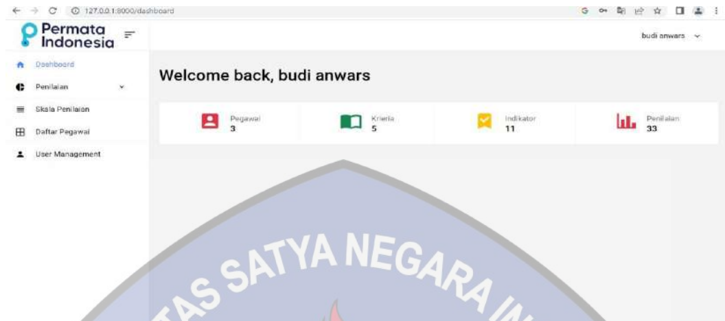
Gambar 4.32 Tampilan Dasboard.
