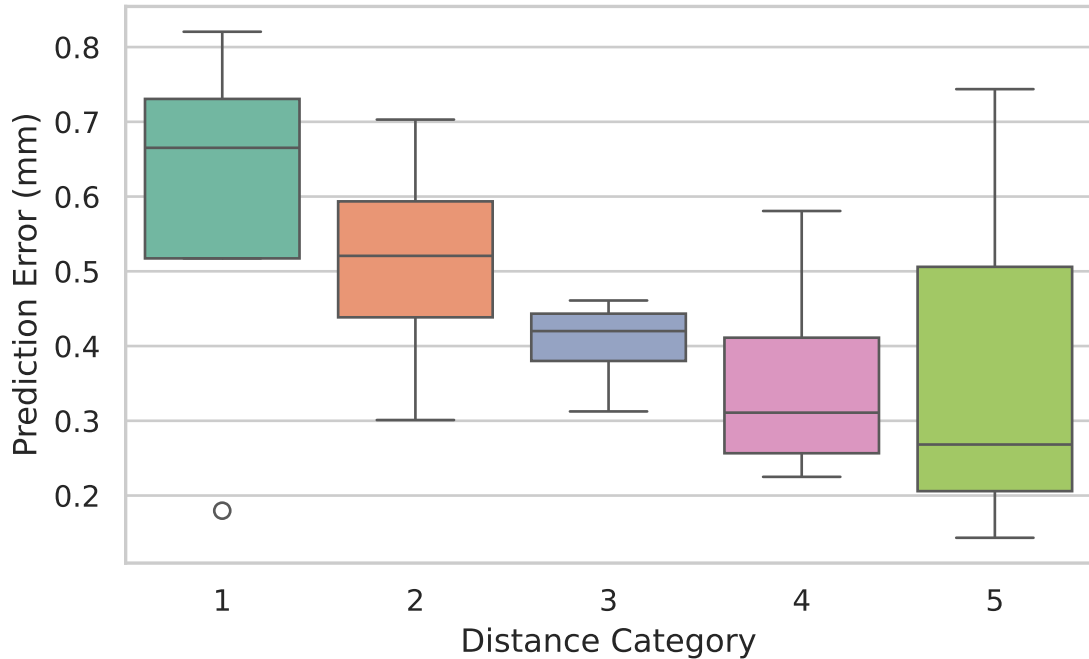
Box Plot of Prediction Errors by Distance Category
