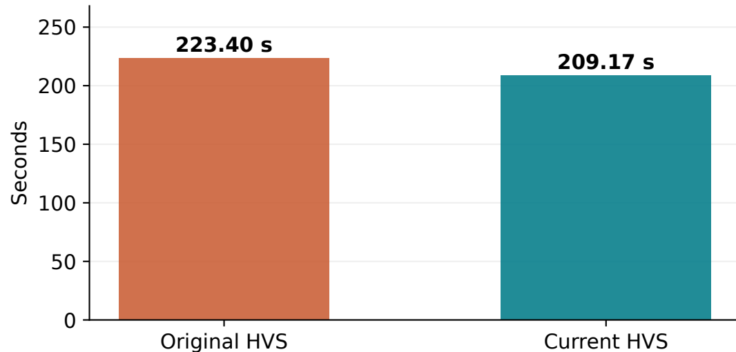
Time until index is query-ready Current: -6.37% time
