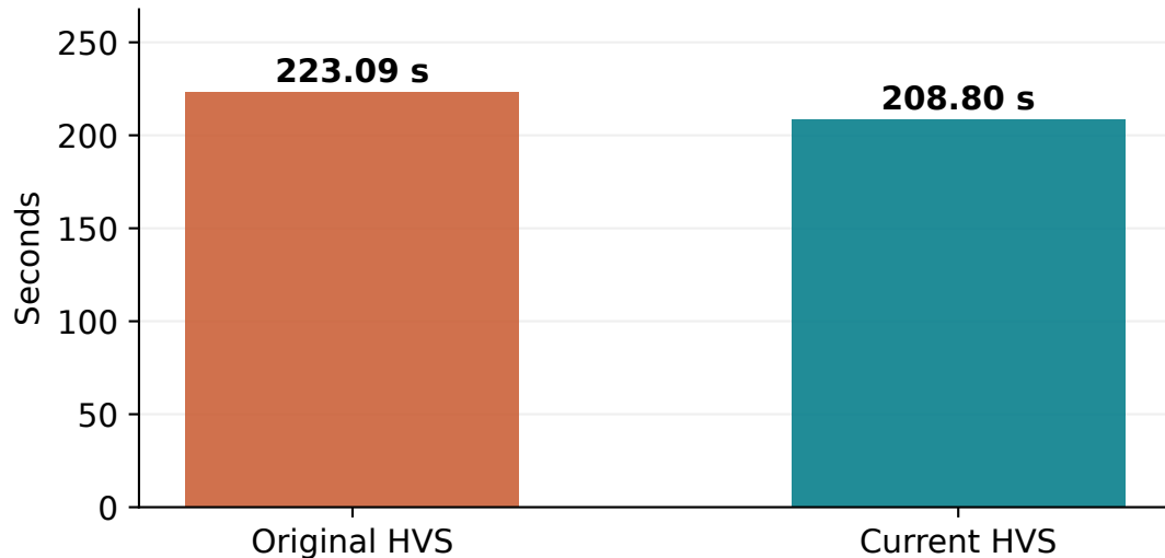
Construction API wall time Current: -6.40% time
