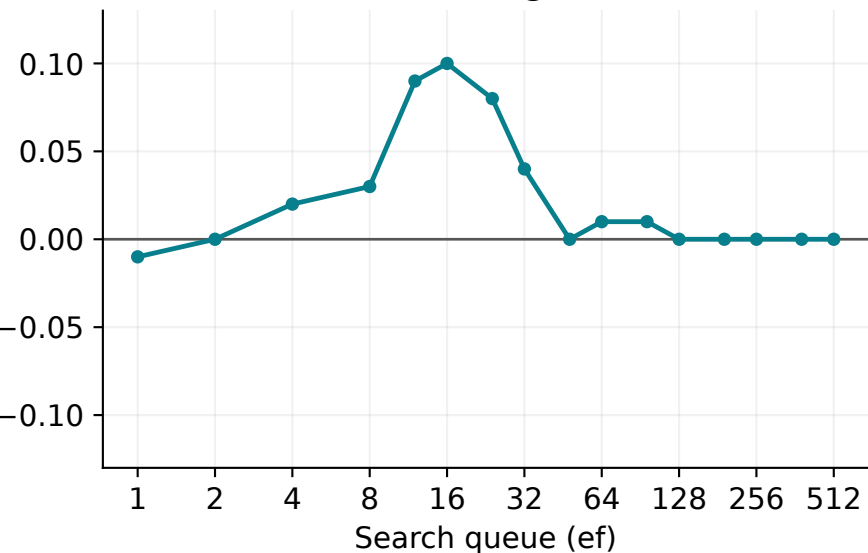
Recall@1
