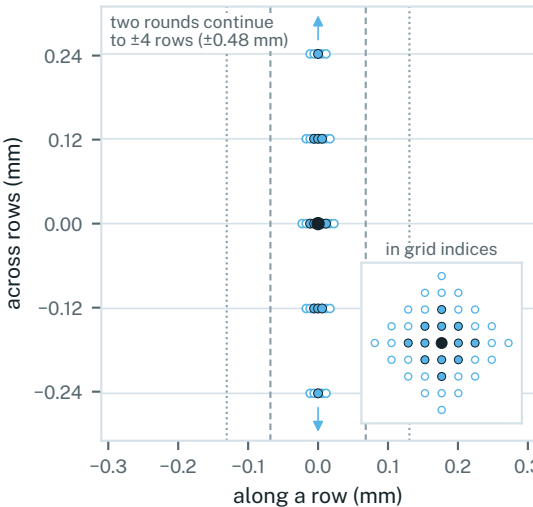
Index-space k-NN graph ( k = 12 )
