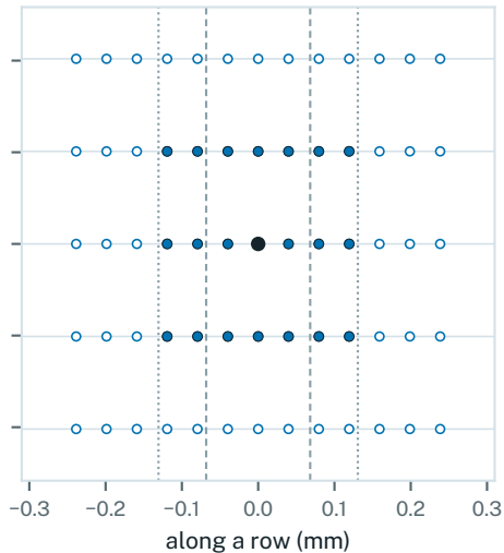
Dilated stencil (20 neighbours)
