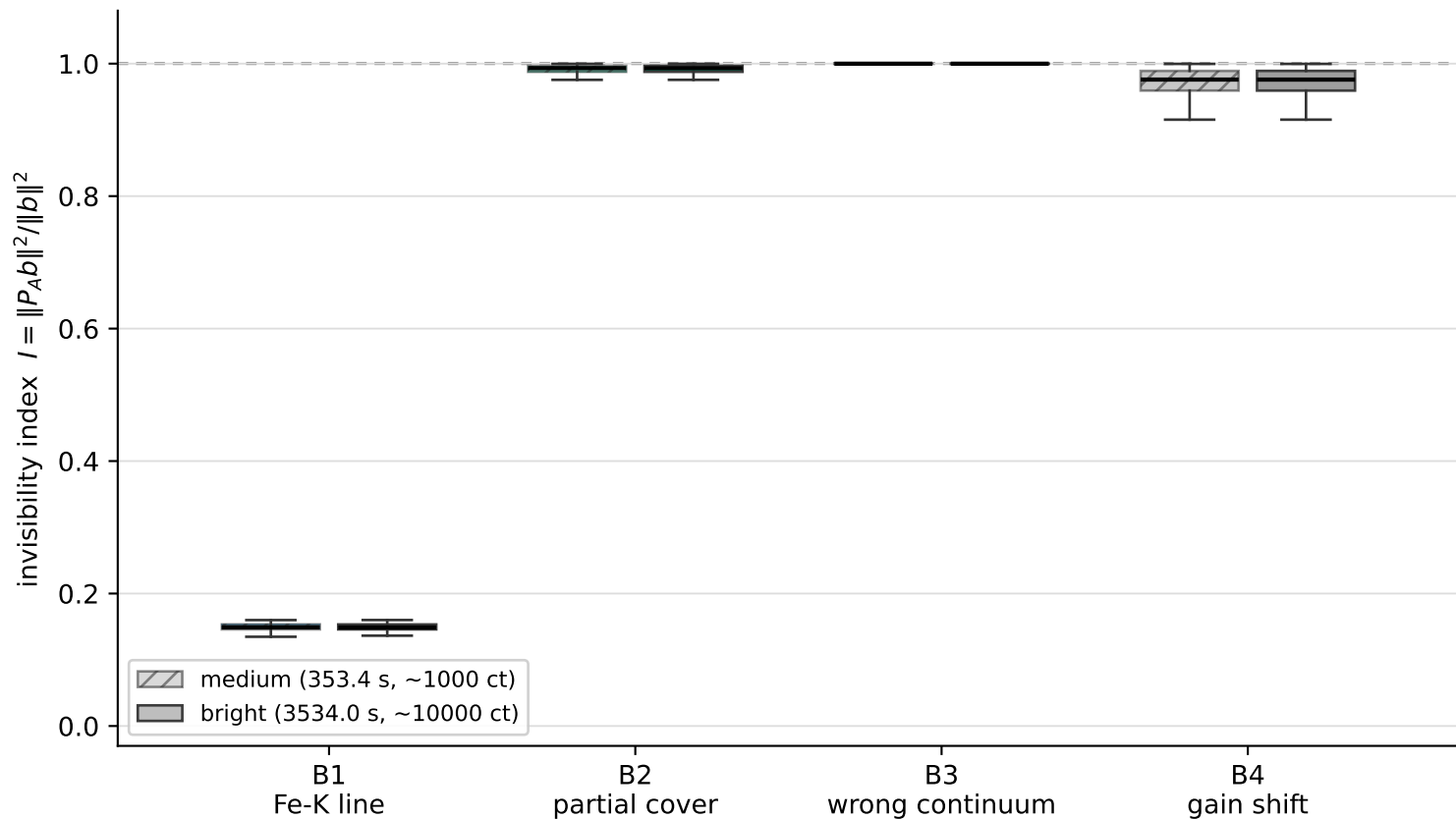
Fisher-metric invisibility index by misspecification family and count level ( I \rightarrow 1 : reabsorbable by refitting \theta ; I \rightarrow 0 : residual survives)
