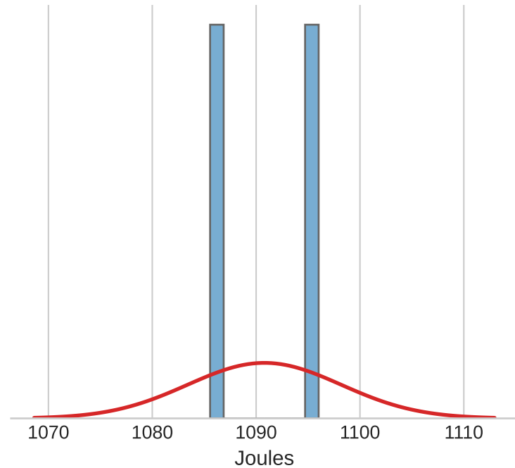
Statistical Distribution
