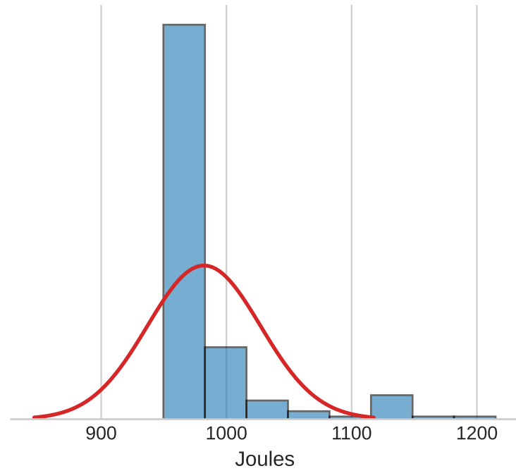
Statistical Distribution
